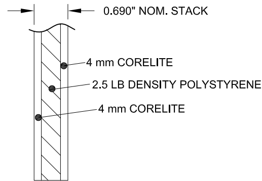
OPAQUE PANEL (OP) MAPES CORELITE ARCHITECTURAL PANEL
